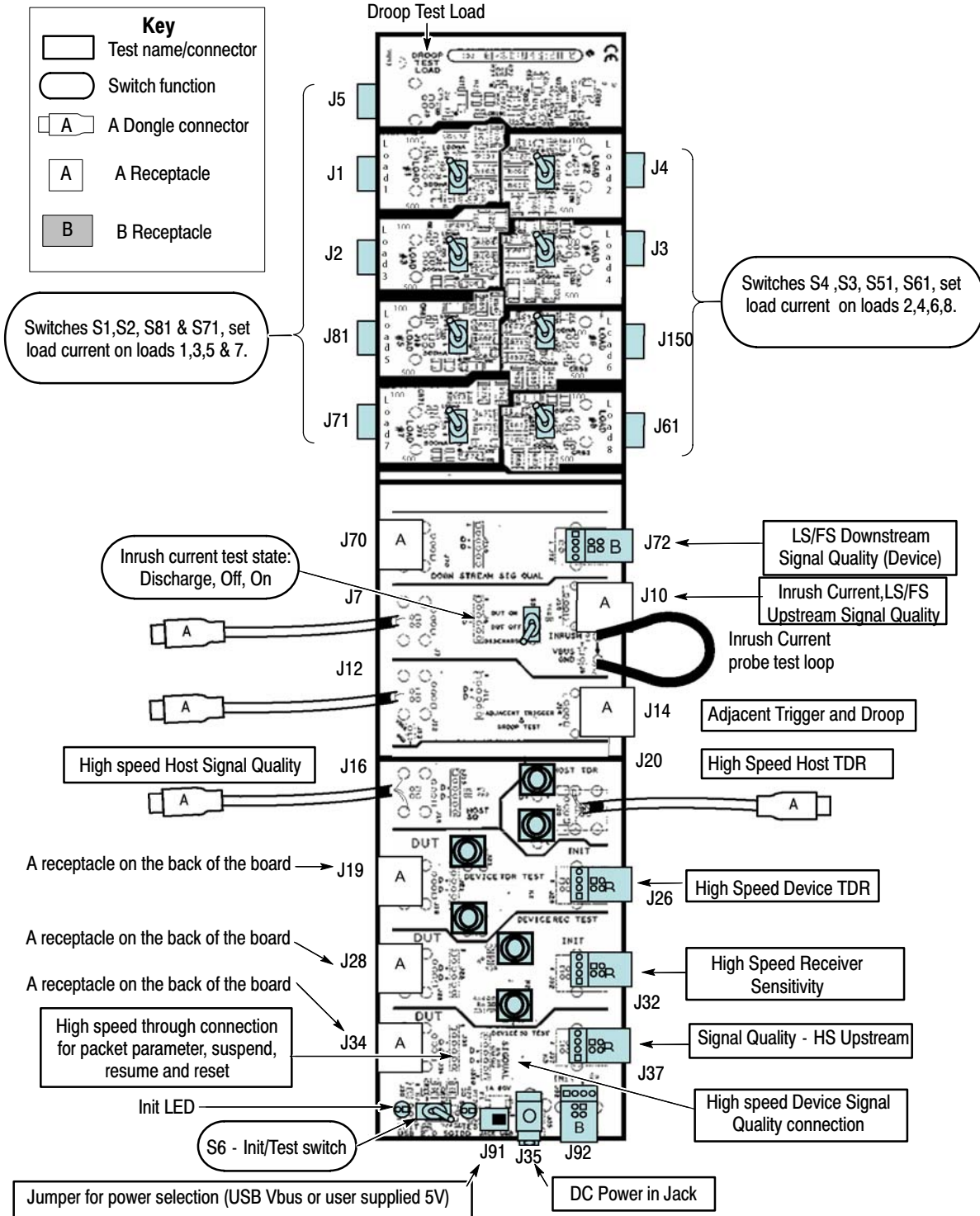
Figure 1: Fixture connections and switch functions
